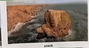
stack
