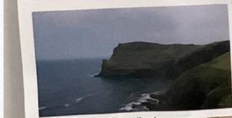
cliff
