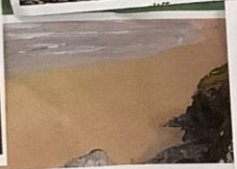
beach
