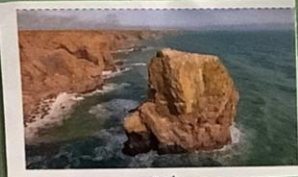
stack
